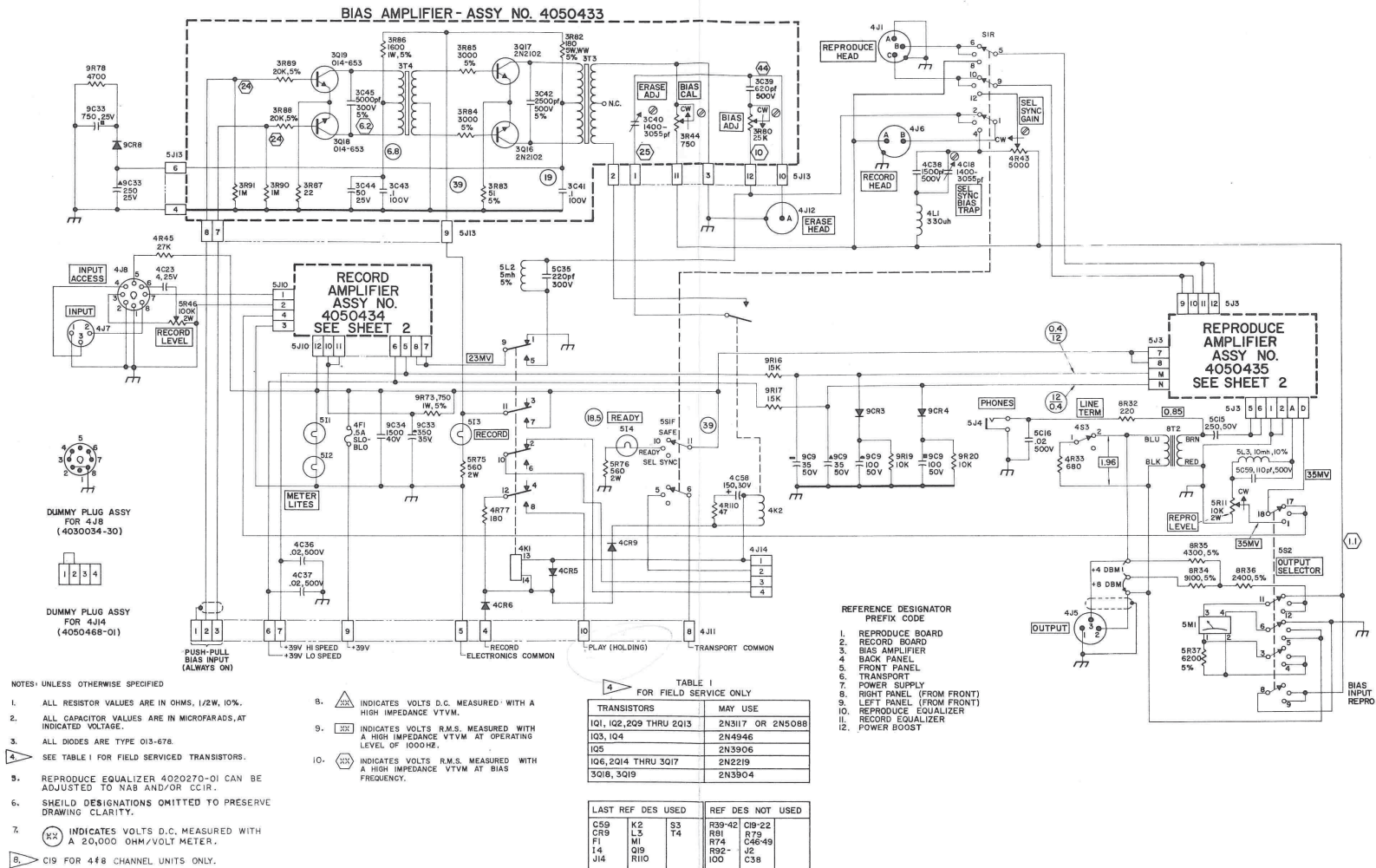
Fig. 6-24A. Schematic Diagram, Electronics
