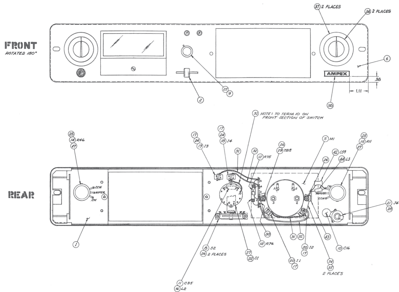
Fig. 6-27. Front Panel Assembly
