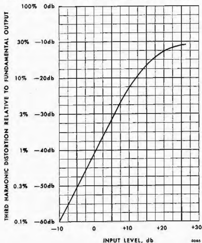
Typical third harmonic distortion vs. input level at 400 cps, measured at 15 ips. Distortion is plotted on a db scale to obtain a logarithmic function in linear steps.
