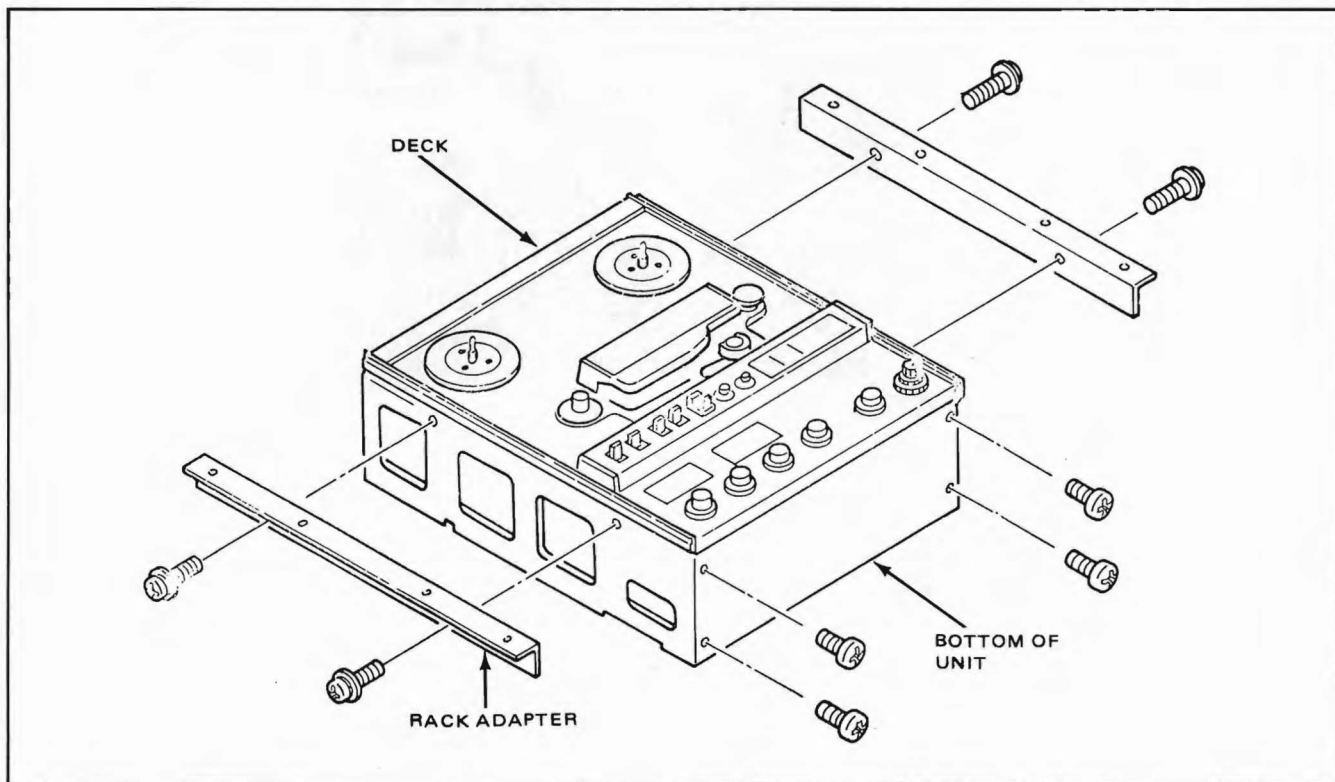
Figure 2-3. Rack Adapter Installation
