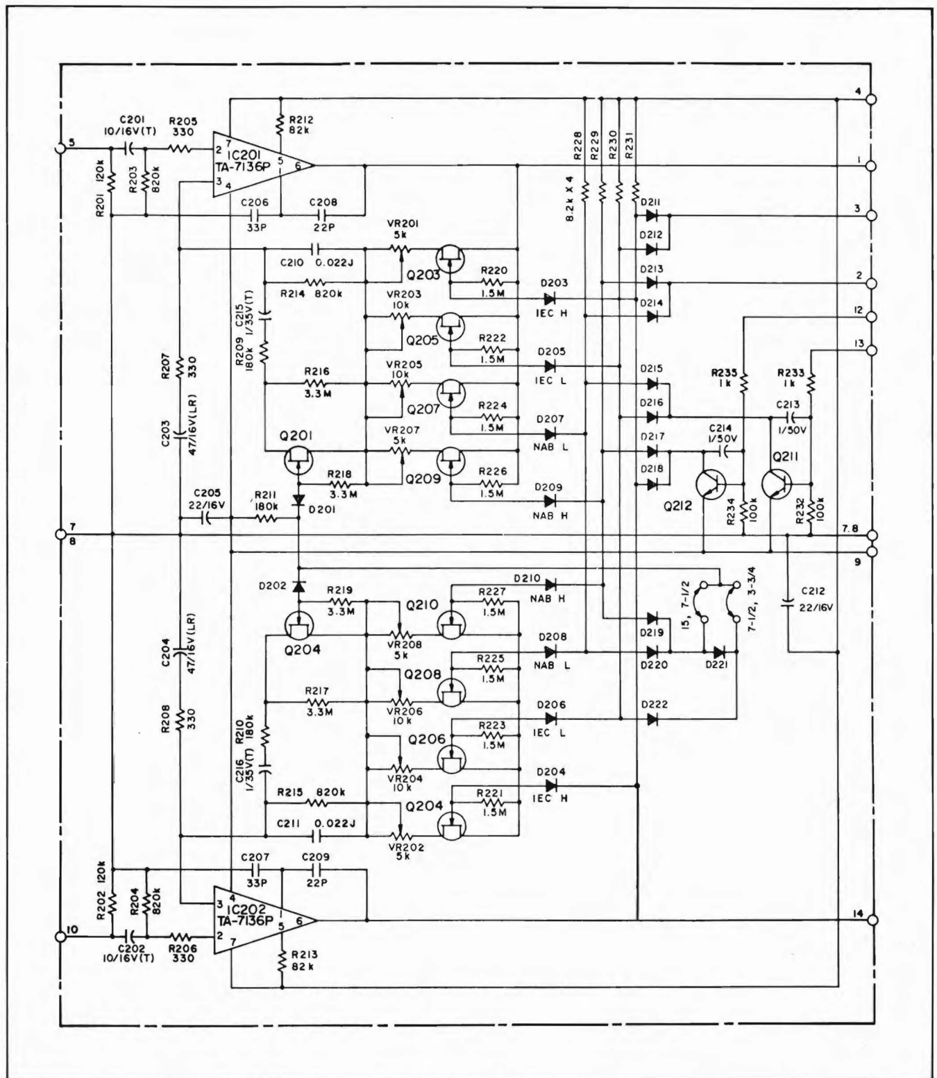
Figure 4-7. Reproduce Equalizer Amplifier Schematic
