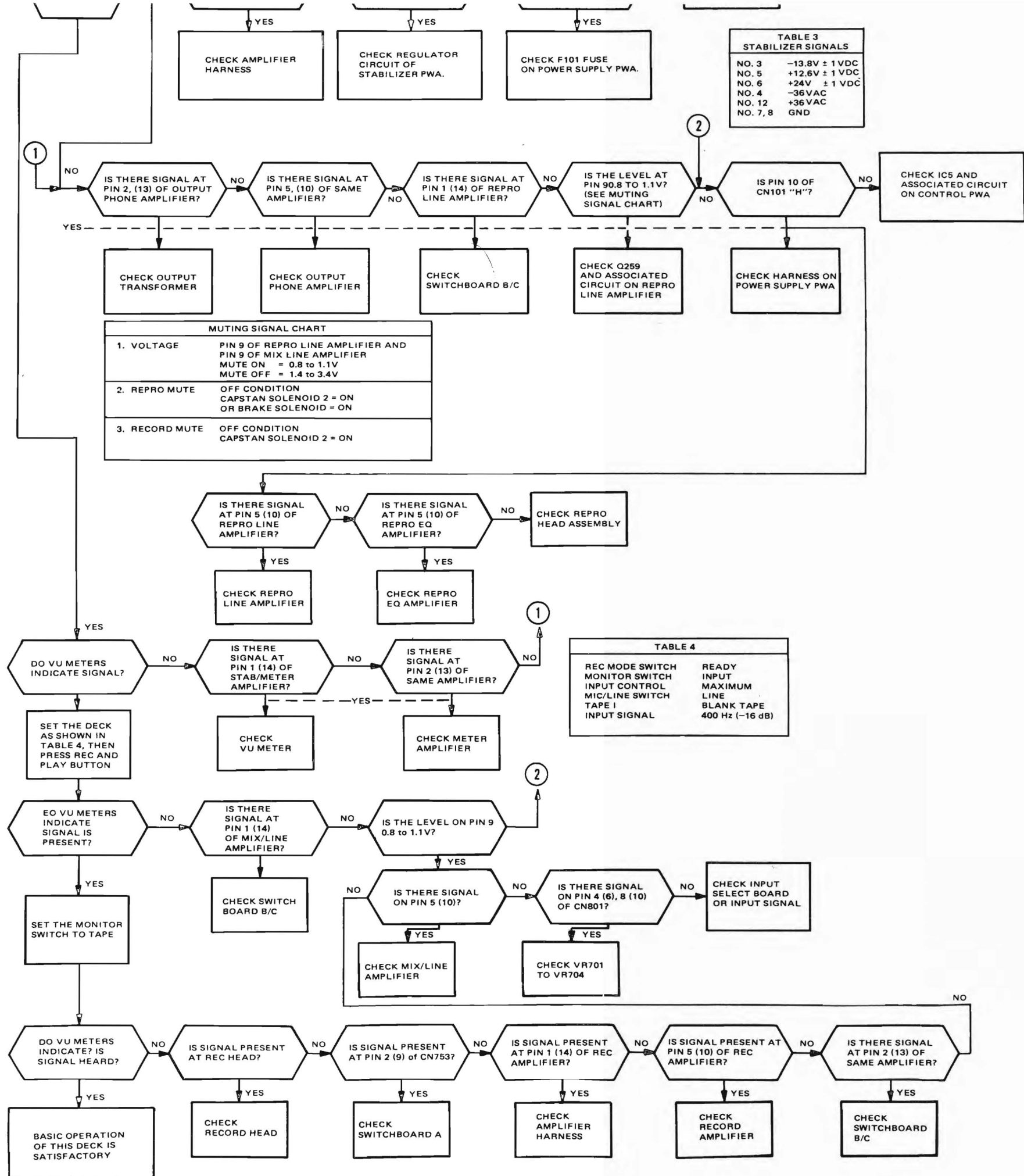
Figure 5-29. Troubleshooting Flow Chart
