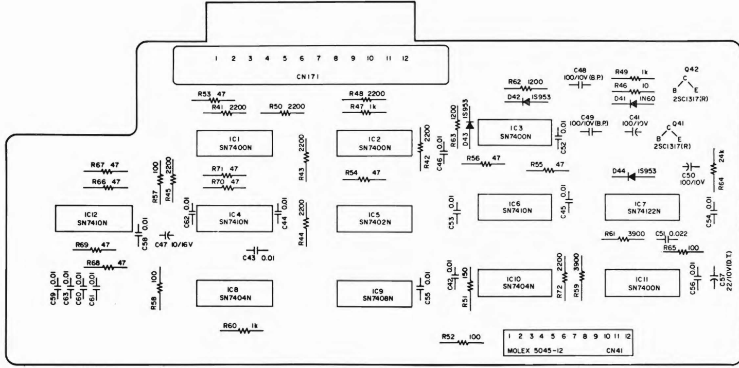
Assembly No. 1418941 Control Unit PWA
