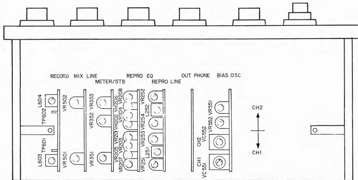
(BOTTOM VIEW OF UNIT — SUPPORT BRACKET REMOVED)
