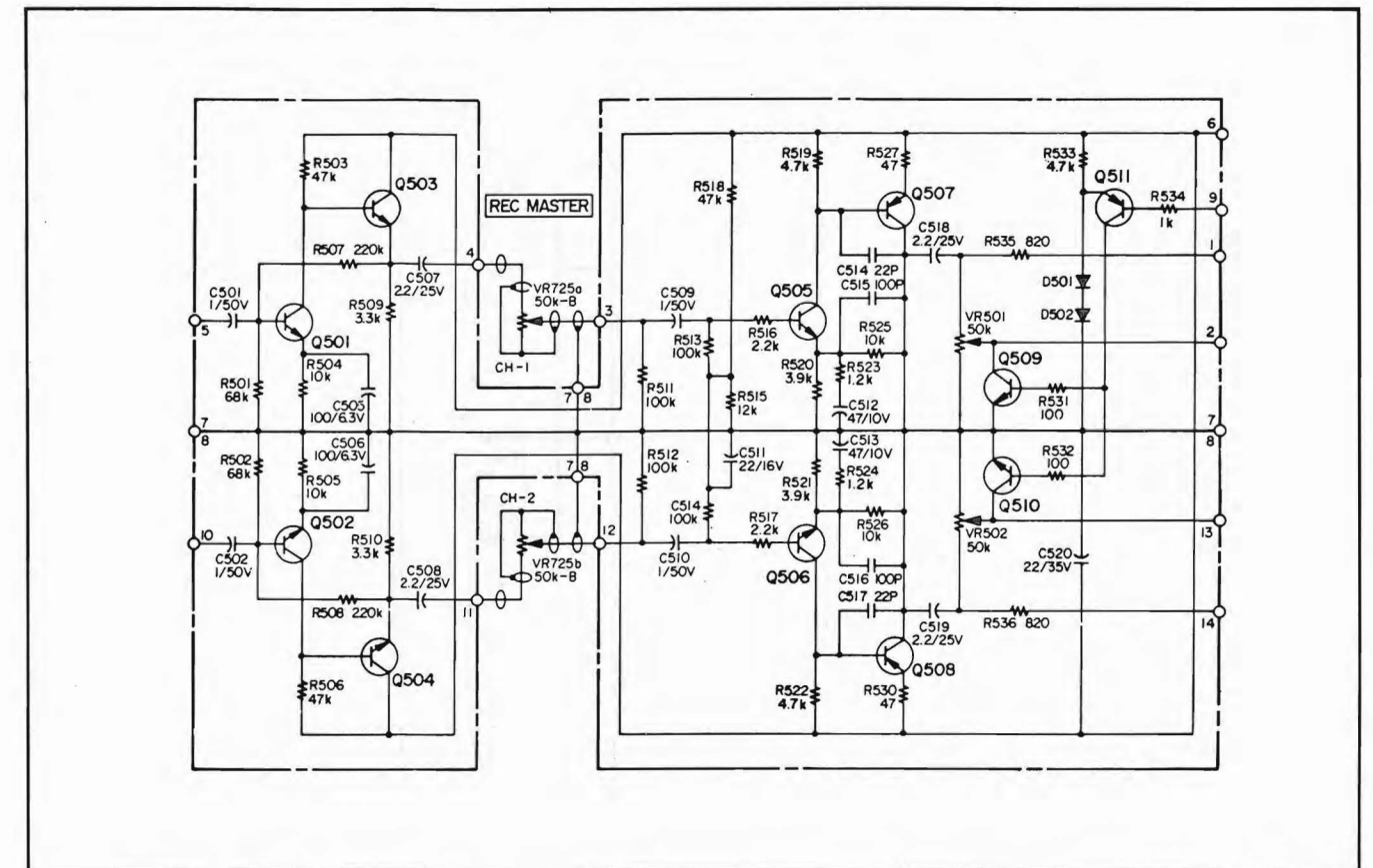
Figure 4-12. Mix Line Amplifier Schematic
