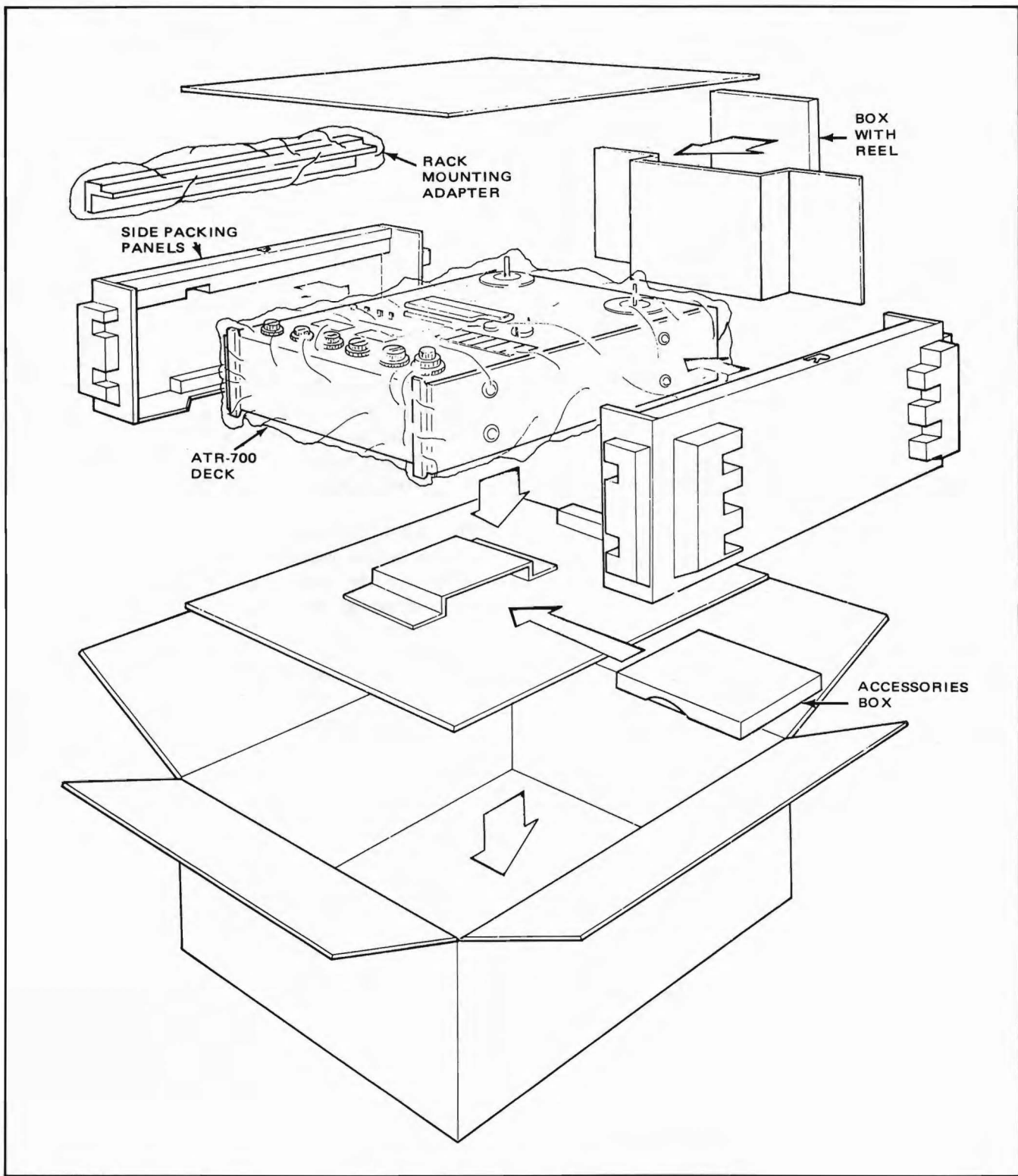
Figure 2-1. Unpacking the ATR-700
