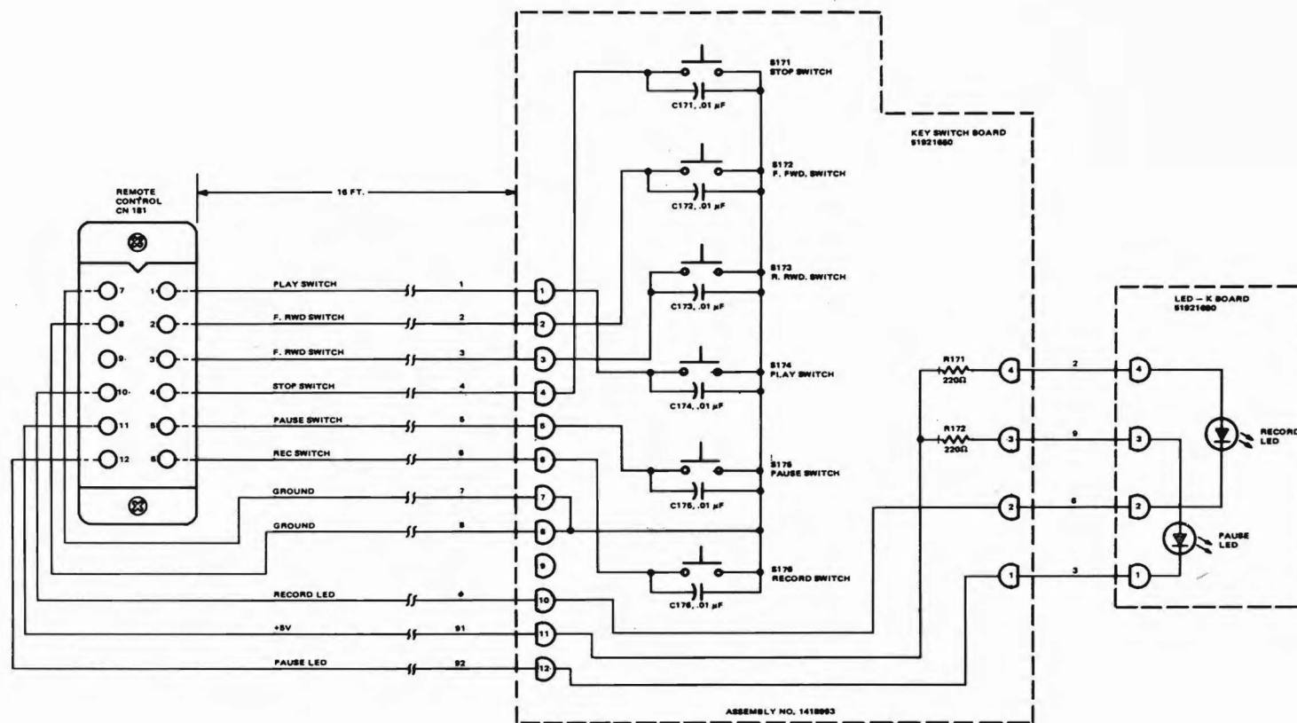
Schematic No. 1418949 Remote Control Assembly
