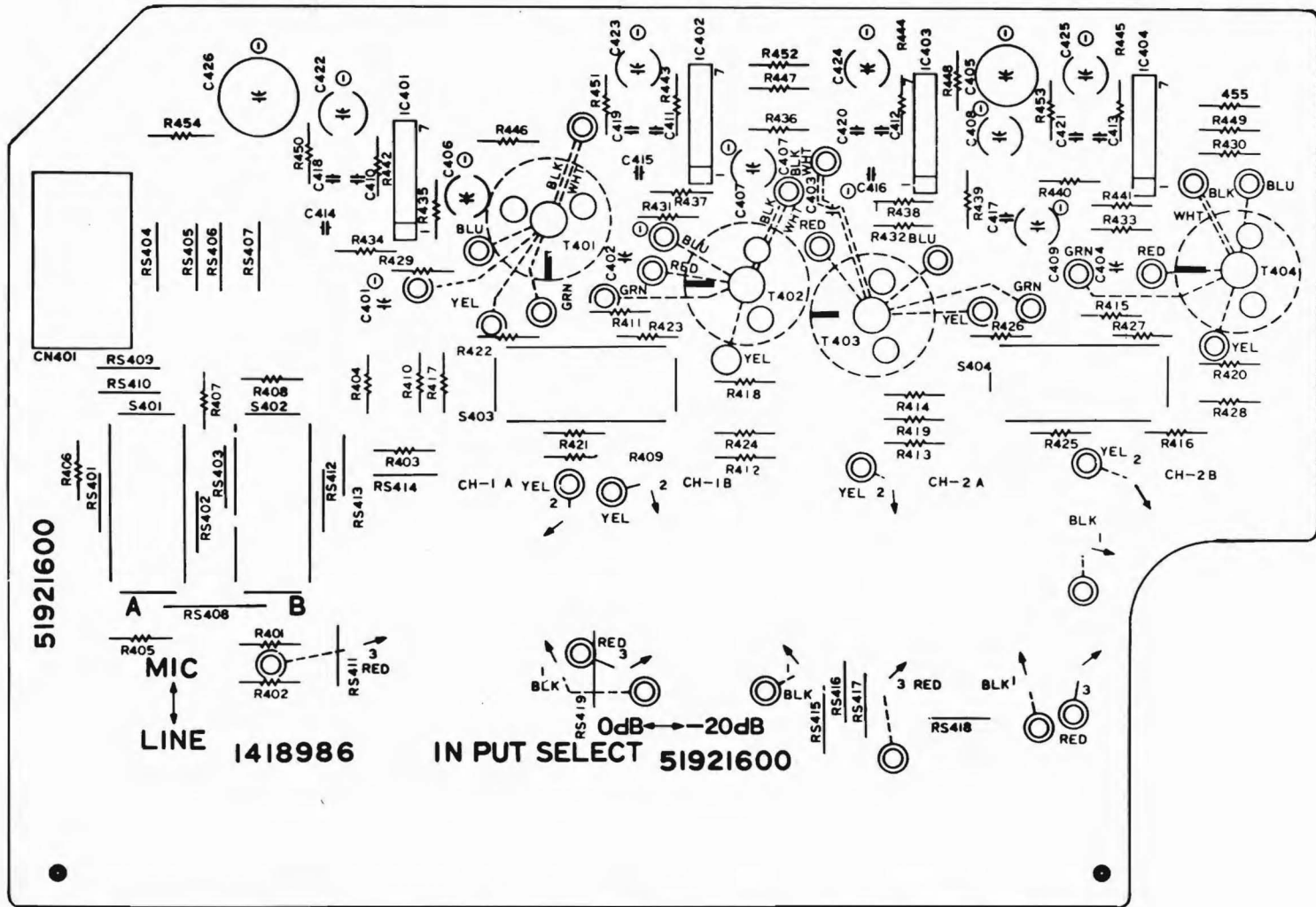
Assembly No. 1418986. Input Select PWA
