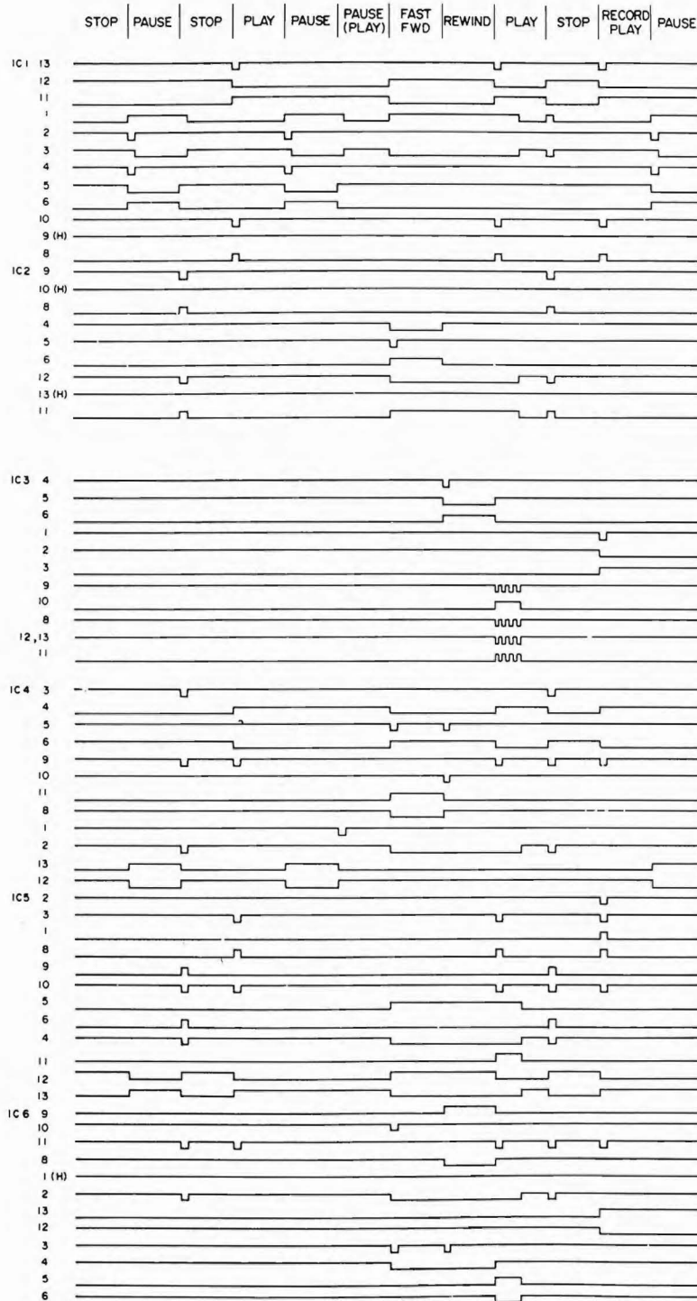
Figure 4-3. Timing Diagram (Sheet 1 of 2)
