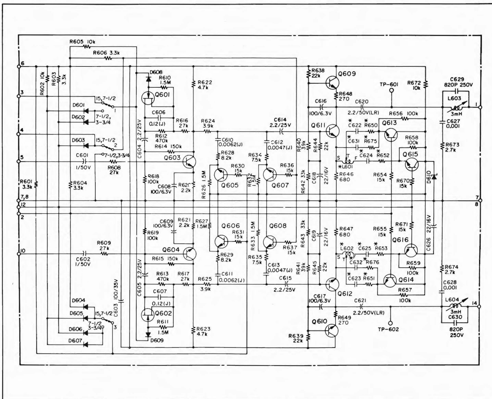
Figure 4-13. Record Amplifier Schematic
