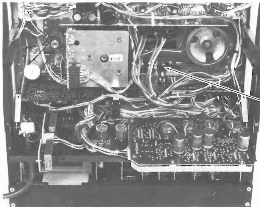
PINCH ROLLER SOLENOID MOUNTING SCREWS (3)
