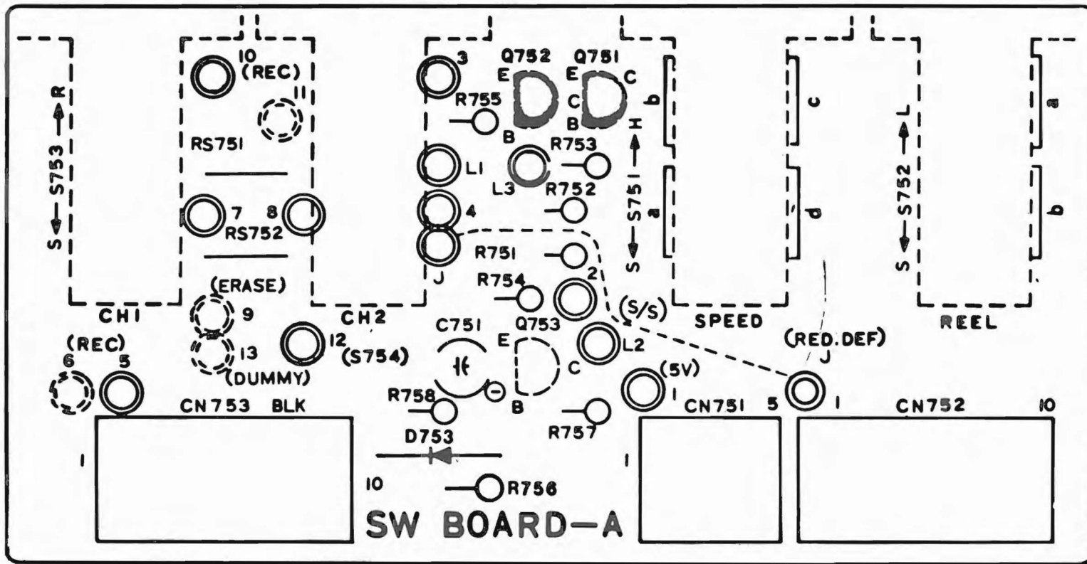
Assembly No. 1418944 Switch Board A PWA
