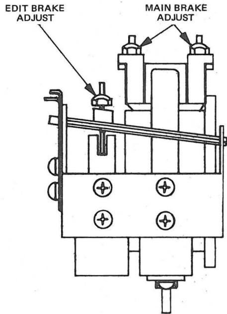
Fig. 4C-2. Brake Adjustments
