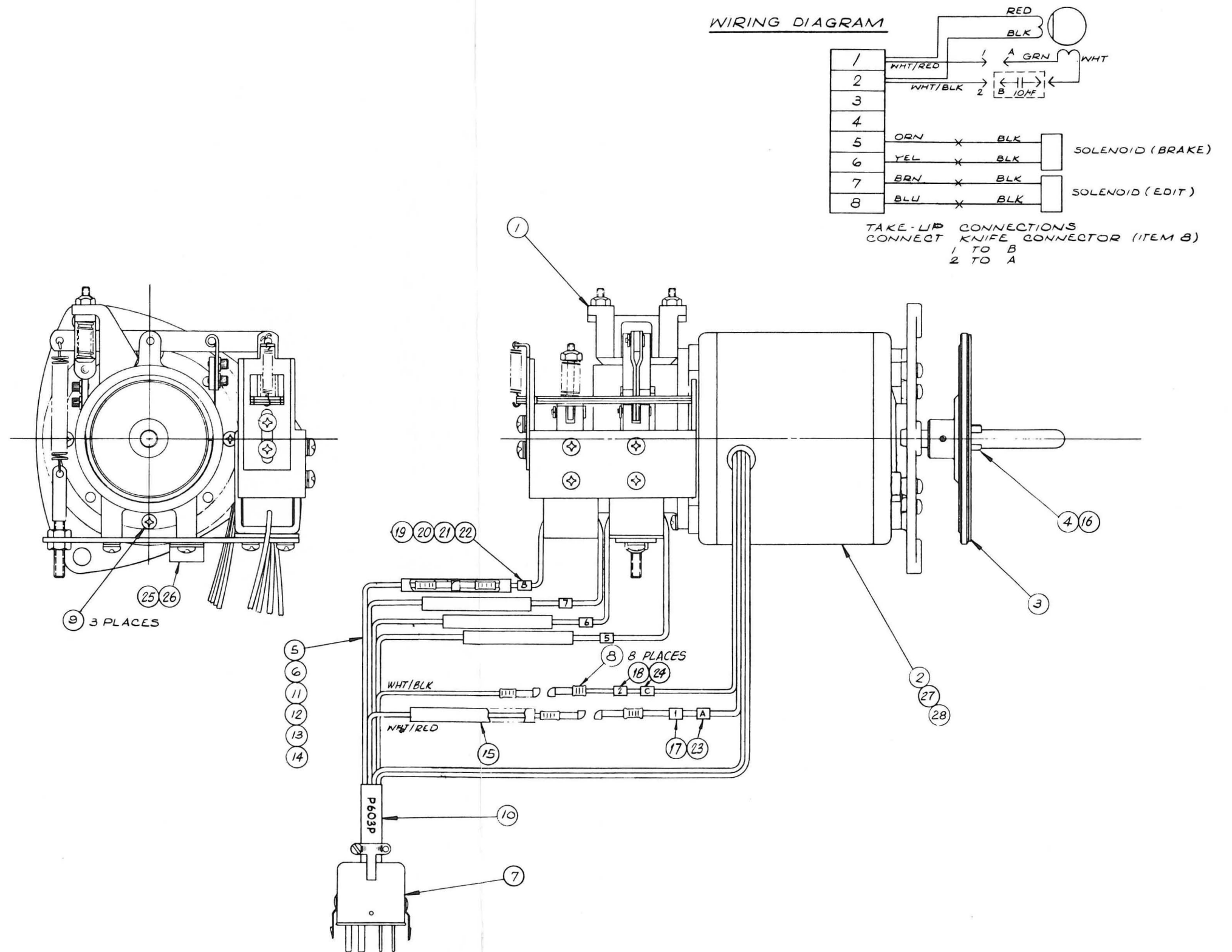
Fig. 6-12. Take-up Assembly
