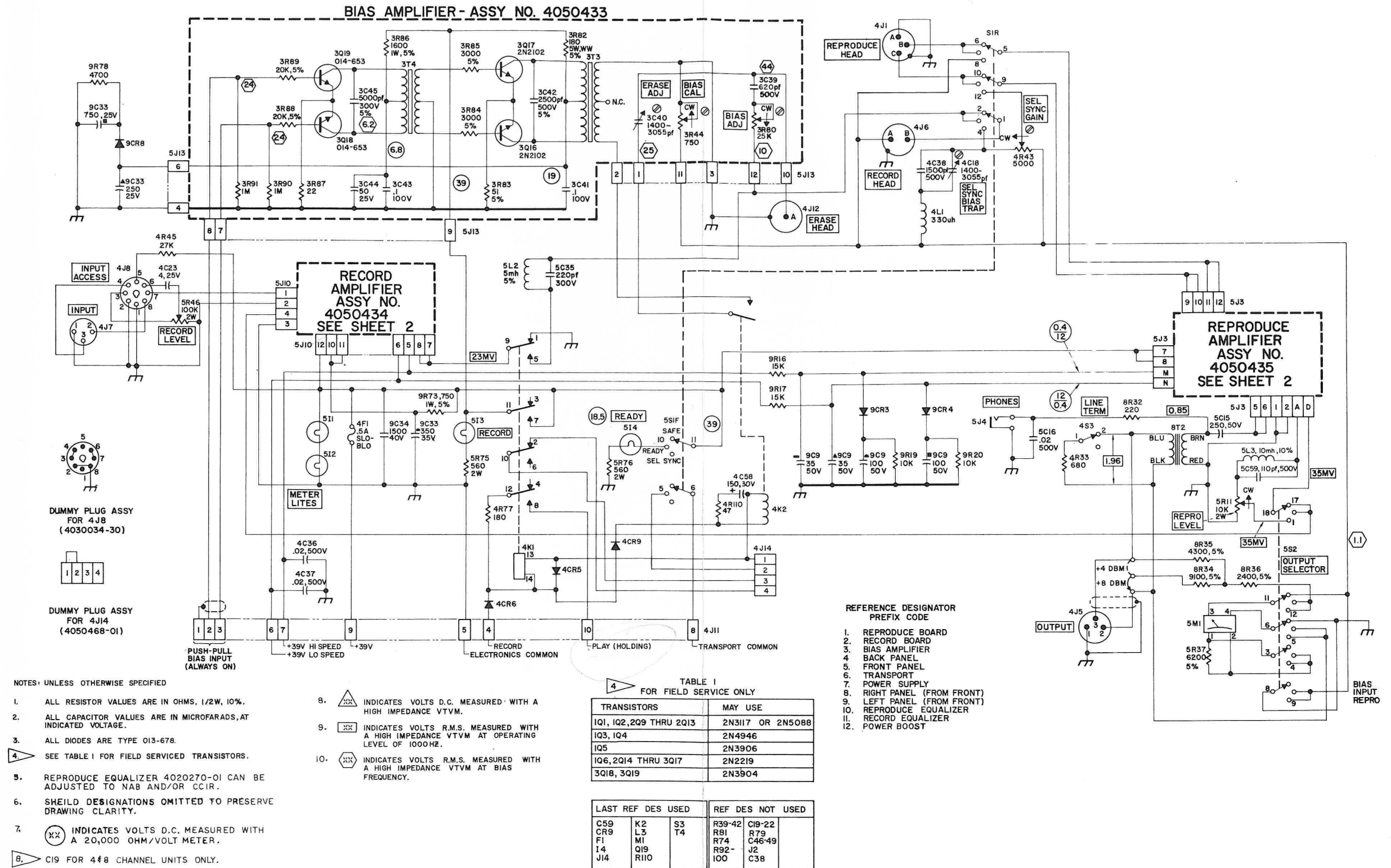
Fig. 6-24A. Schematic Diagram, Electronics
