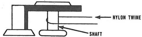
Fig. 4C-4. Capstan Idler Force Measurement
