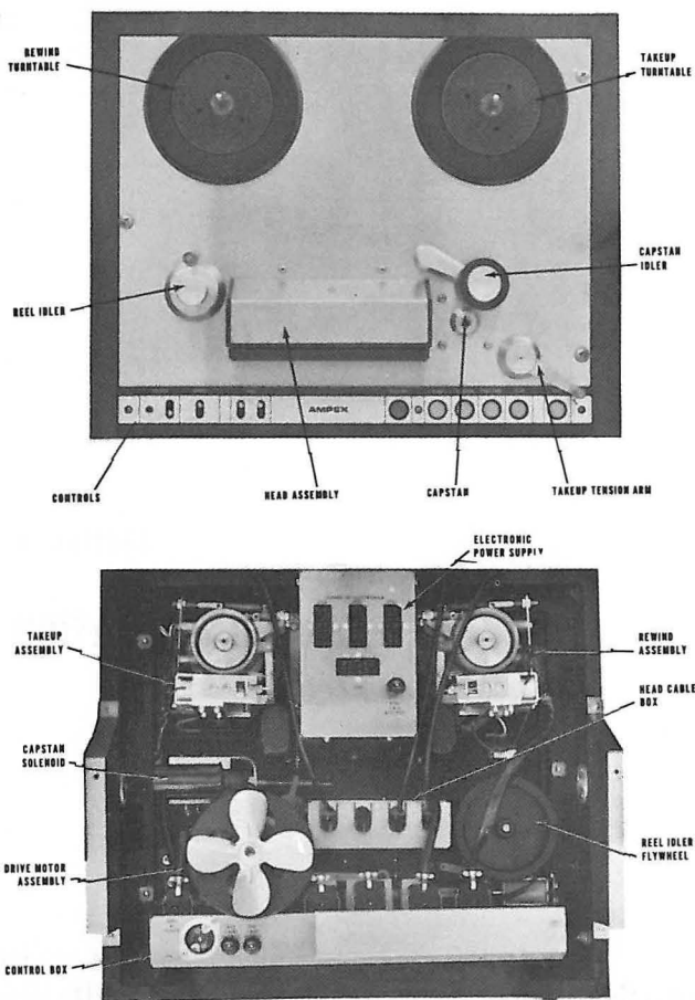
Fig. 5-1. Tape Transport
