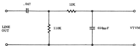
Fig. 4B-1. Noise Filter Schematic
