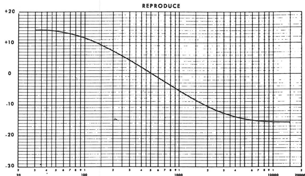
Fig. 6-32. Response Curves, Sheet 1
