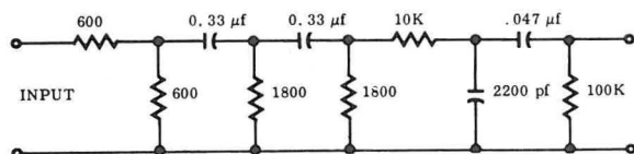
Fig. 4B-2. ASA "A"-Curve Filter Schematic 04773
