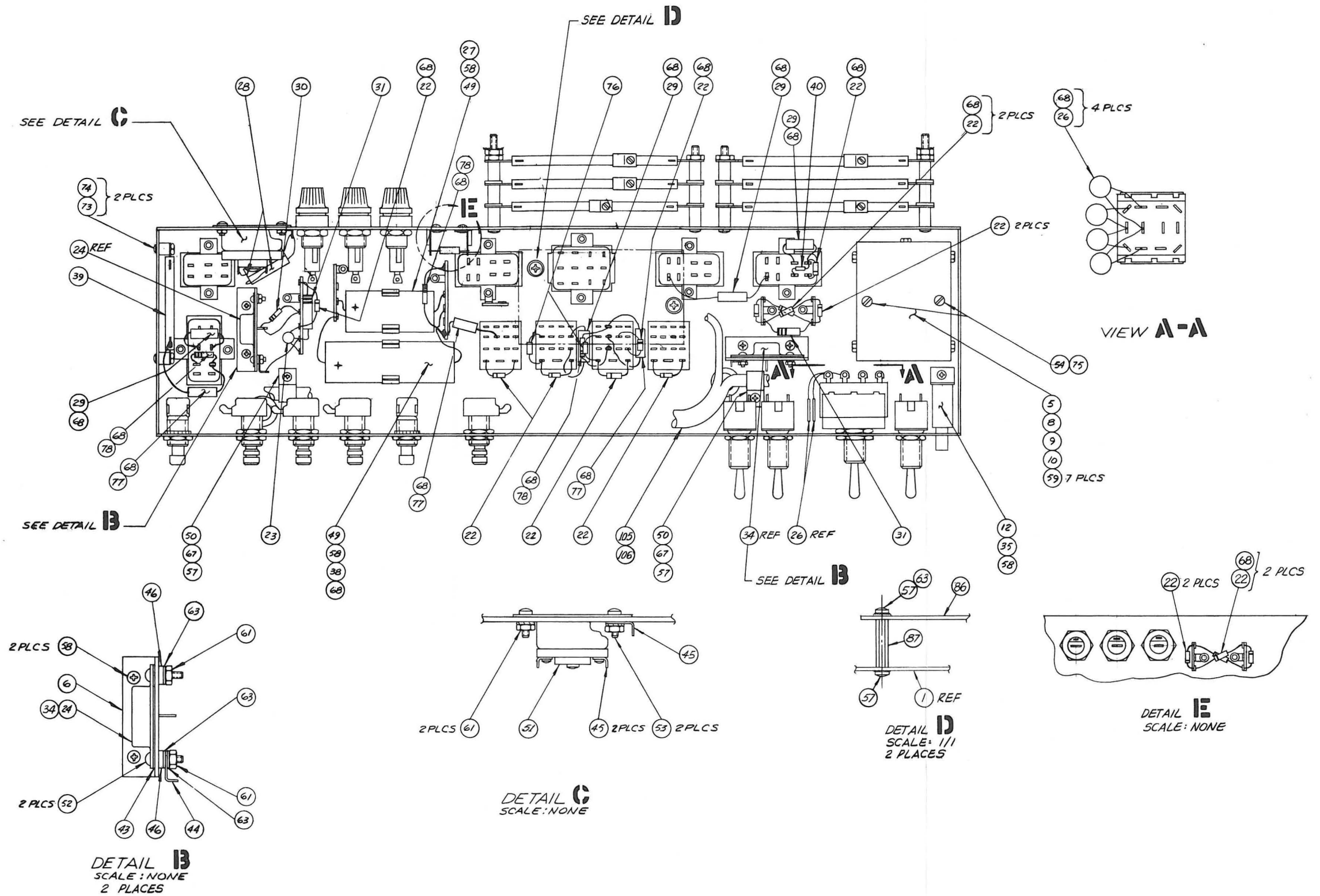
Fig. 6-18. Control Box, Inner
