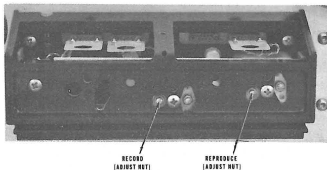
Fig. 4C-6. Head Azimuth Adjustments
