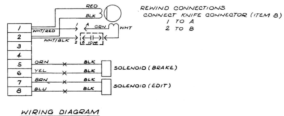
Fig. 6-13. Rewind Assembly
