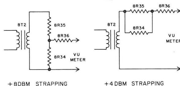
Fig. 5-3. Strapping Circuit, Simplified
